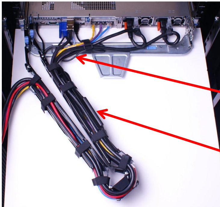
Figure 4. Routing the cables through the CMA
